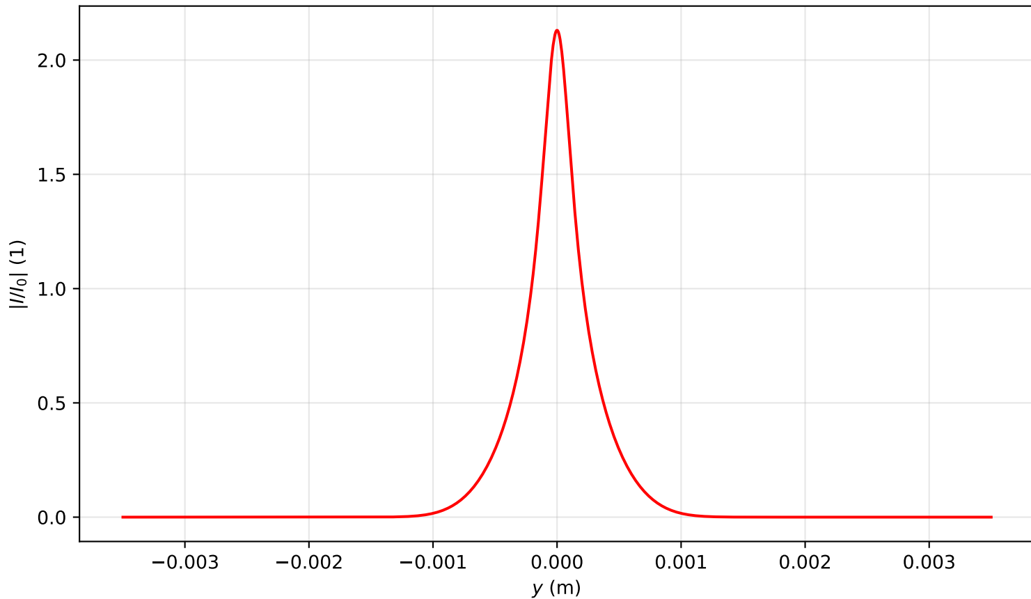
Intensity profile I(x = 0, y, z = 0.239)/I_0 , P_{in}=8.5P_{cr} , artificial time
